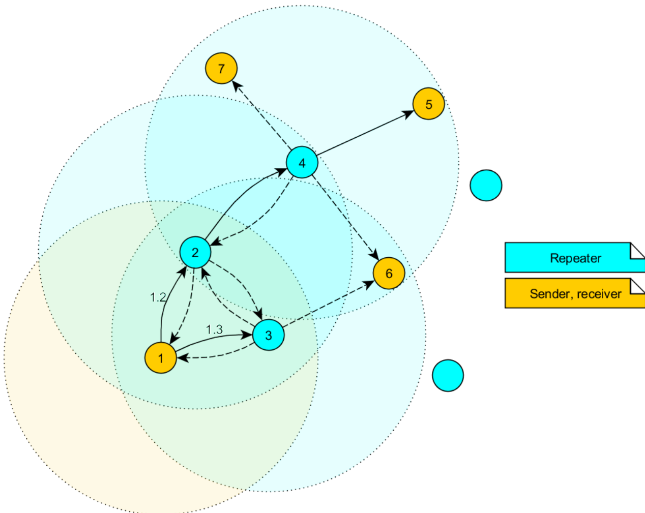
Figure 7: Example network
