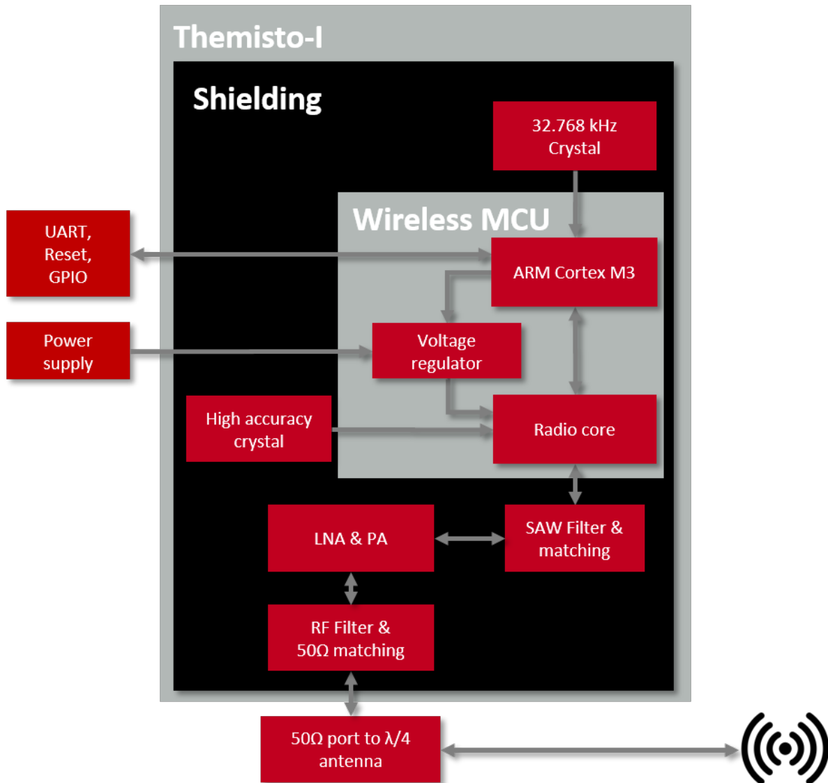
Figure 1: Block diagram
