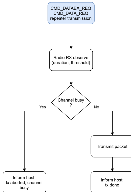
Figure 8: Listen Before Talk
